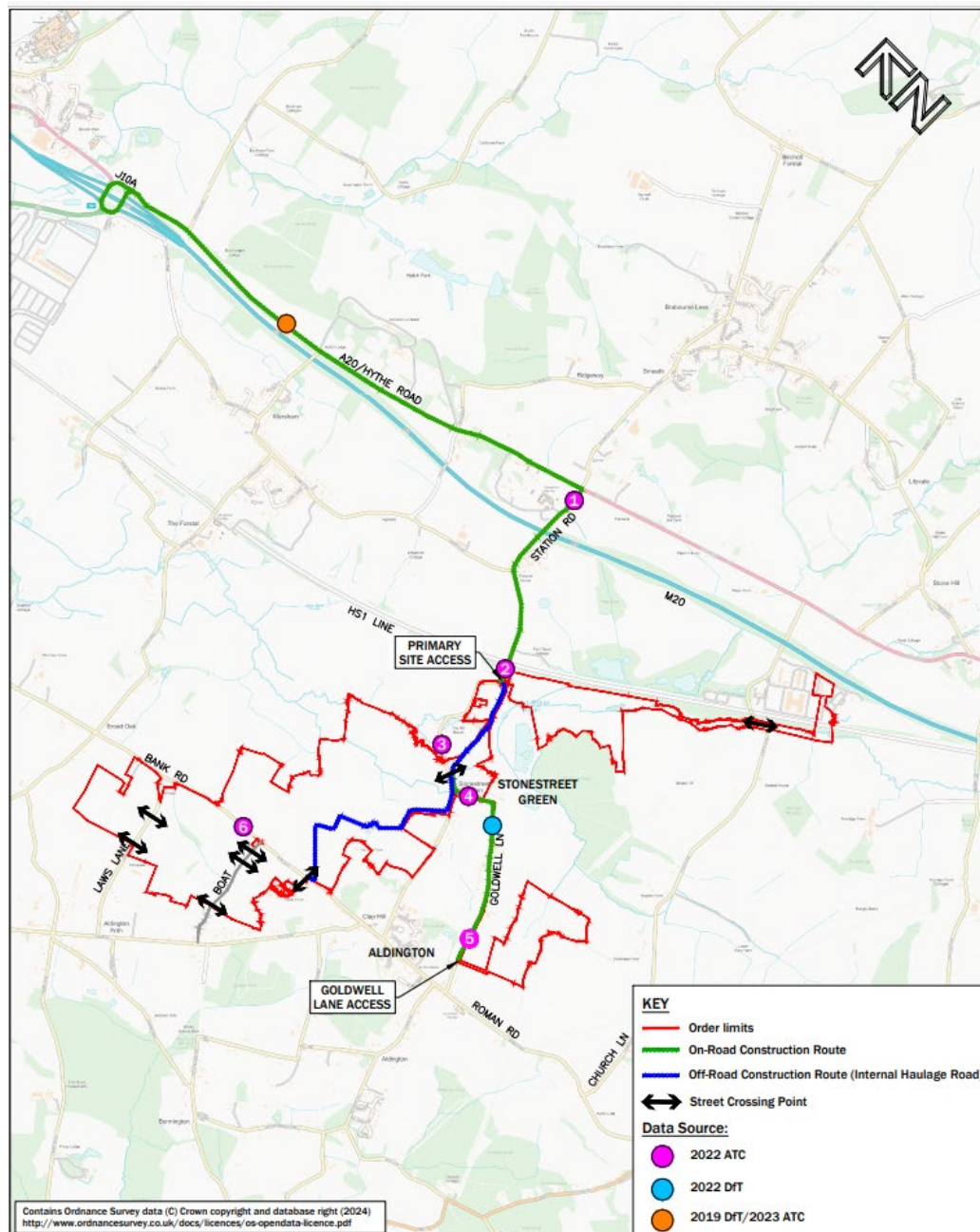
Figure 4 Construction internal haulage route
